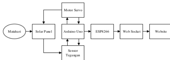
Gambar 1 Block diagram sistem
